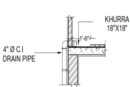
KHURRA SECTION DETAIL (A)
